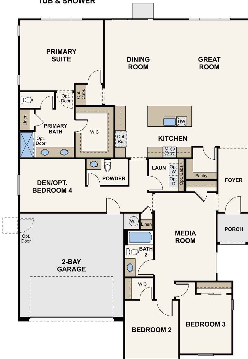
FLOOR PLAN
